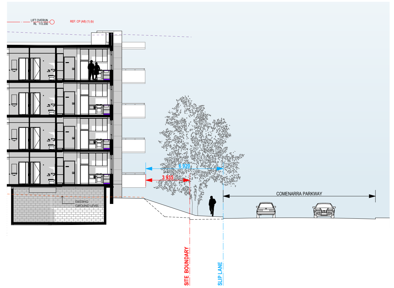
SECTION F - SLIP LANE SECTION
